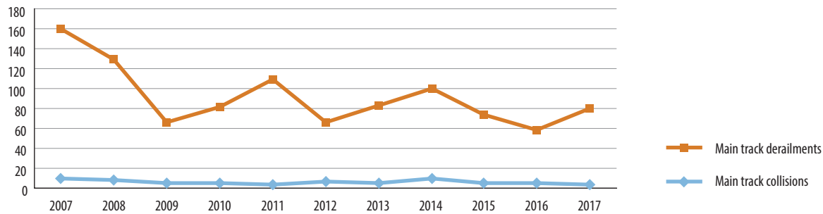
FIGURE 3: MAIN TRACK DERAILMENTS AND COLLISIONS FROM 2007-2017
