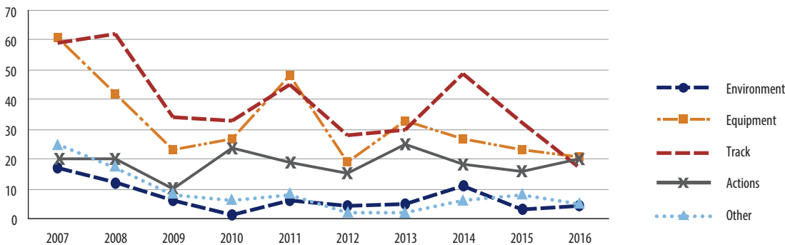
FIGURE 5: ASSIGNED FACTORS IN MAIN TRACK DERAILMENTS, 2007-2016 22
