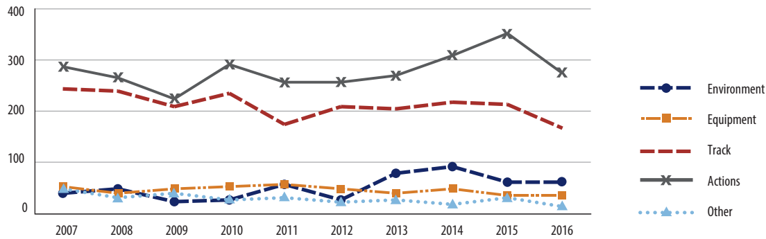
FIGURE 6: ASSIGNED FACTORS IN NON-MAIN TRACK DERAILMENTS, 2007-2016 23
