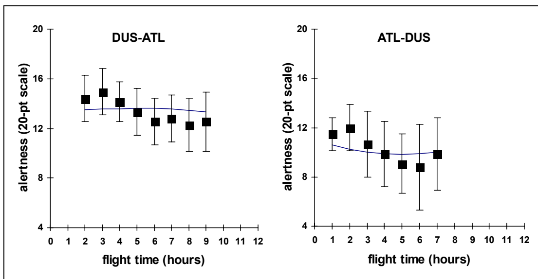
Figure 14 Observed (squares) and Predicted (continuous line) Alertness on the Atlanta Trip
